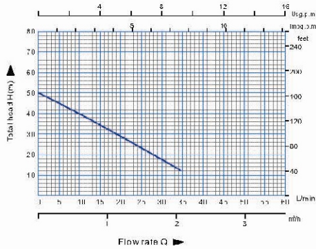
PERFORMANCE CHART AT n=2850RPM
