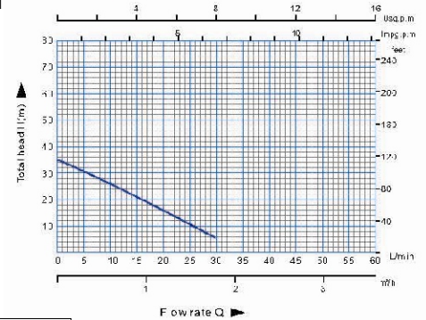
PERFORMANCE CHART AT n=2850RPM
